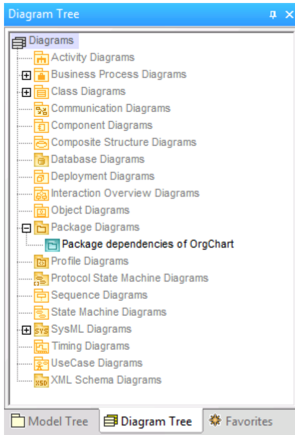
Diagram Tree
