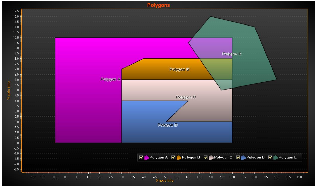
Figure 6-64. Several polygons.
