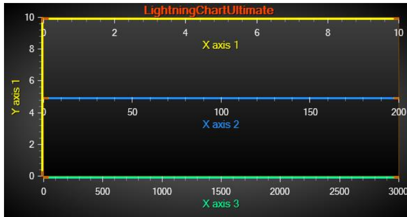
Figure 6-9. XAxisAutoPlacement = Off. Automatic axis placement is disabled, and Position and Alignment properties of each axis apply separately. First axis Position = 0, Second axis Position = 50 and Third axis position = 100.
