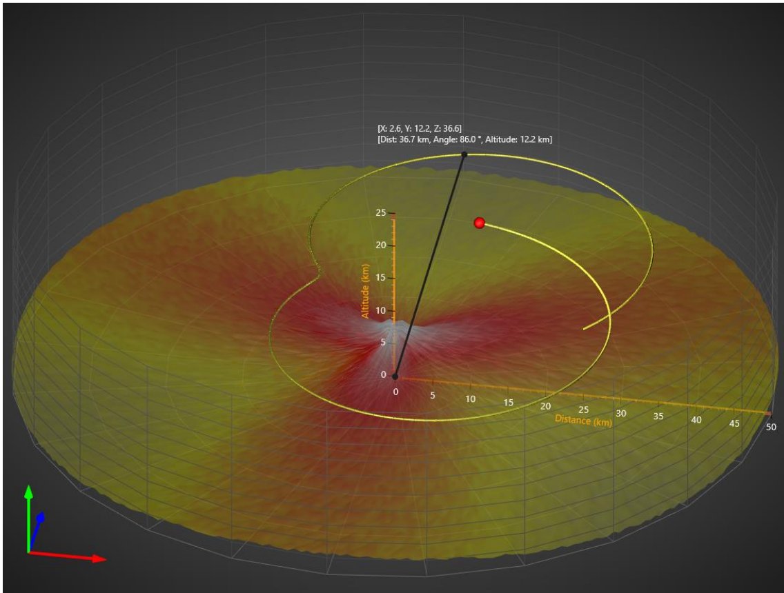
Figure 8-2. Example created with CylindricalCartesian3D converter. Data points of SurfaceMeshSeries3D and the grid are defined in cylindrical coordinates. Annotation tracks the nearest data point of a PointLineSeries3d and displays its value in cylindrical coordinates.
